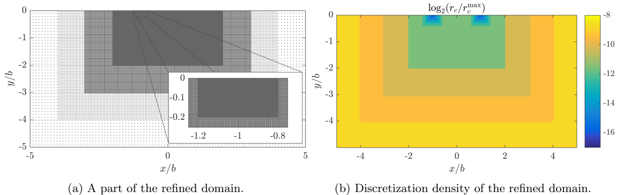
Figure 14: An example of 17-times refined domain used in solution of the described Hertzian contact problem.
