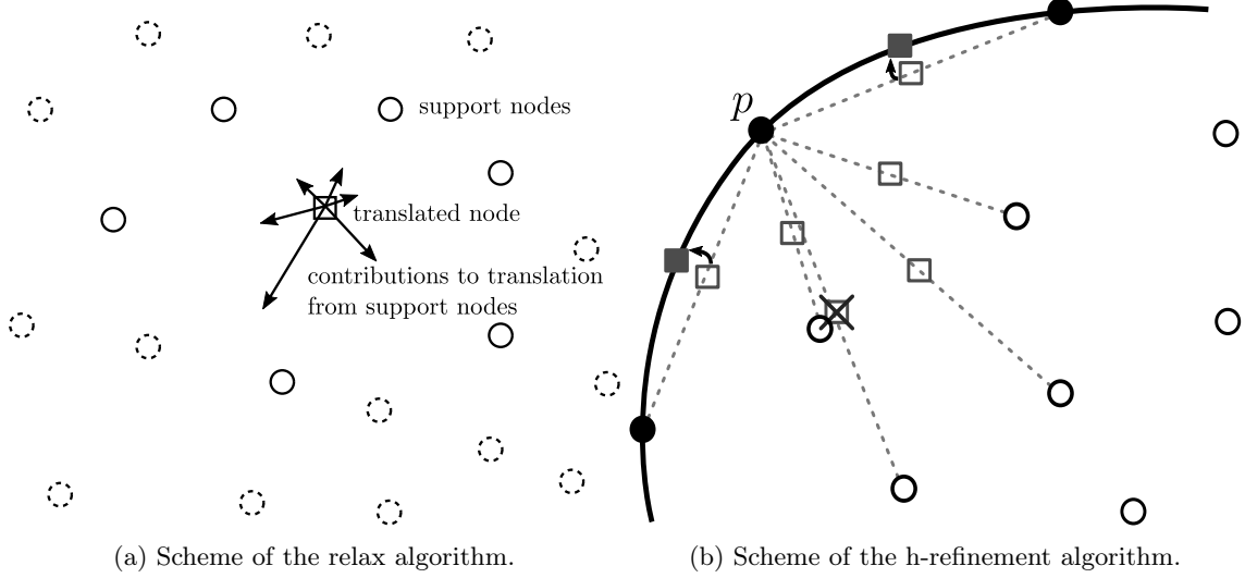
Figure 2: Schemes of algorithms used to improve the quality of the discretization.
