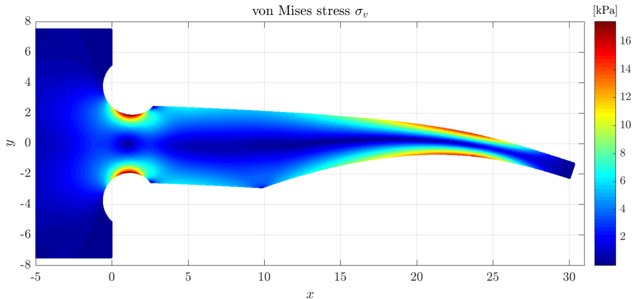
Figure 10: Numerical solution of an irregular cantilever beam using N = 67887 nodes. Note that for the sake of visibility the displacements are multiplied by factor 10^5 .
