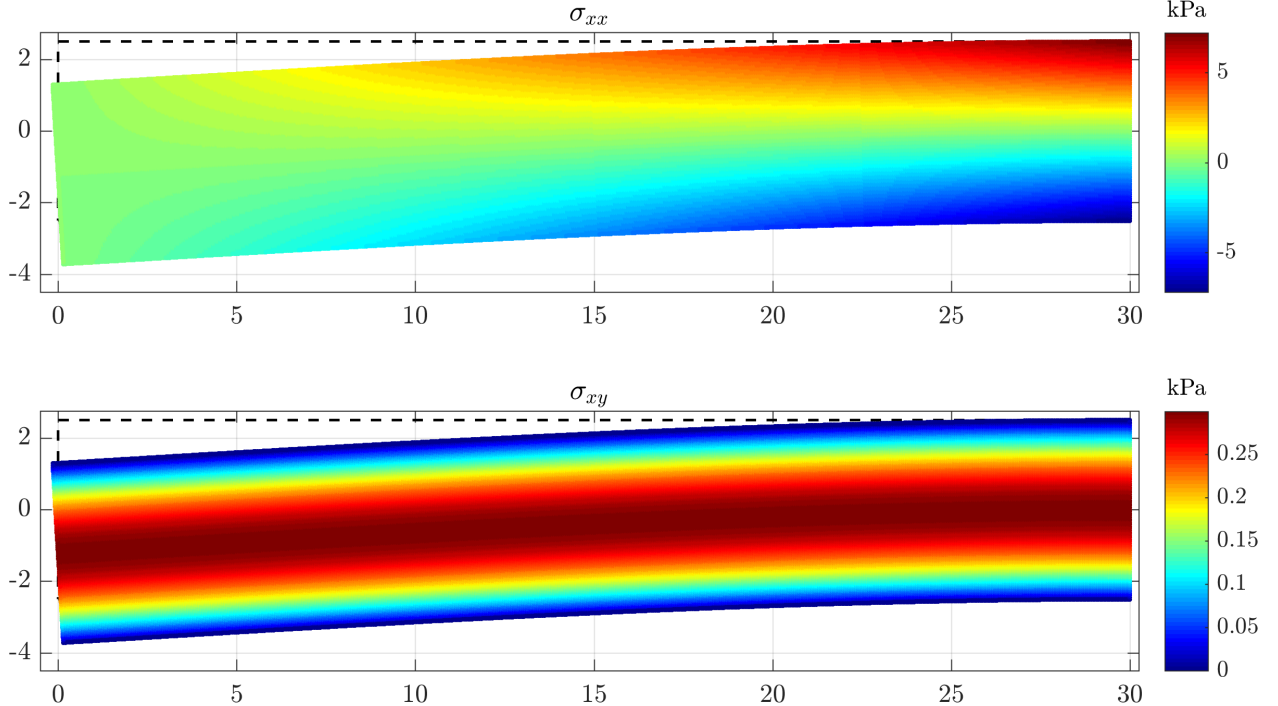
Figure 4: Numerical solution of cantilever beam case. Note that for the sake of visibility the displacements are multiplied by factor 10^5 .
