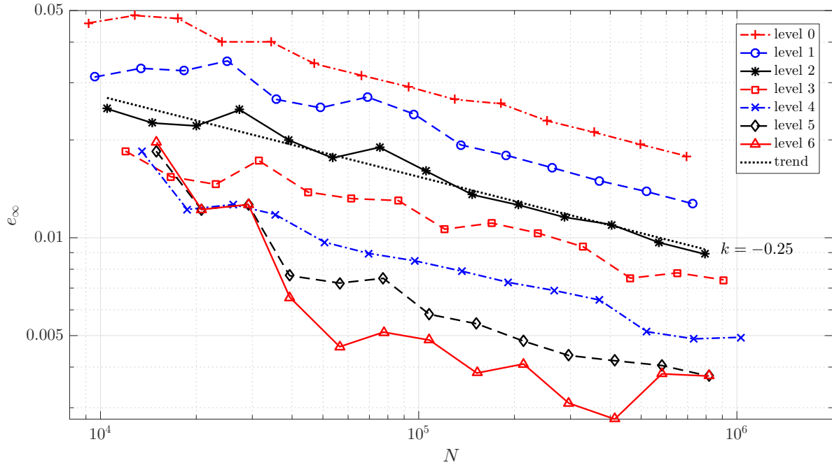
Figure 15: Convergence of MLSM at different refine levels.
