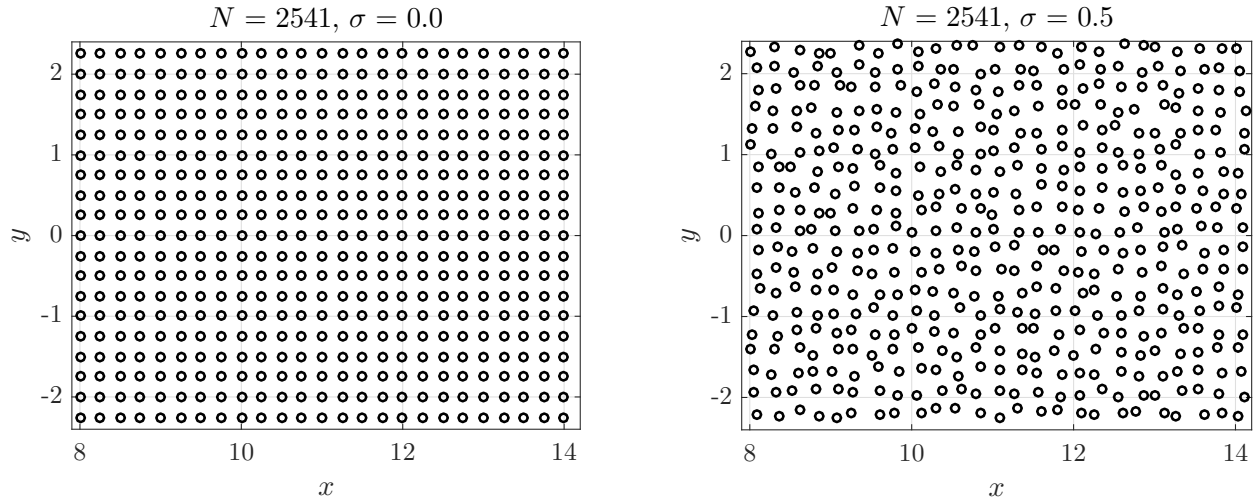
Figure 6: Regular and perturbed node positions, as used in stability analysis.
