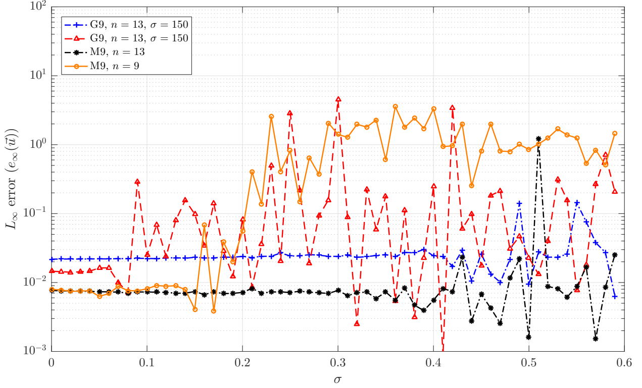
Figure 7: Stability of MLSM with respect to nodal perturbations.
